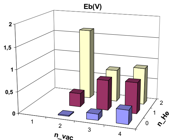
Fig. 6. Binding energy (eV) of a vacancy to small He_m Vac_n complexes in Ni (VASP/PAW results) [22].
